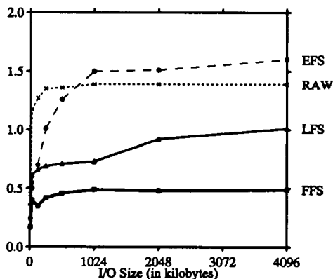
Figure 9: Maximum File System Write Bandwidth.
