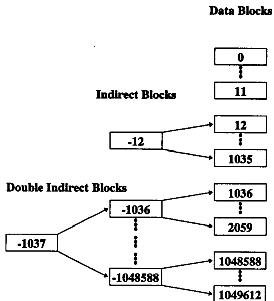
Figure 6: Block-numbering in BSD-LFS. In BSD-LFS, data blocks are assigned positive block numbers beginning with 0. Indirect blocks are numbered with the negative of the first data block that they address. Double and triple indirect blocks are numbered with one less than the first indirect or double indirect block that they address.
